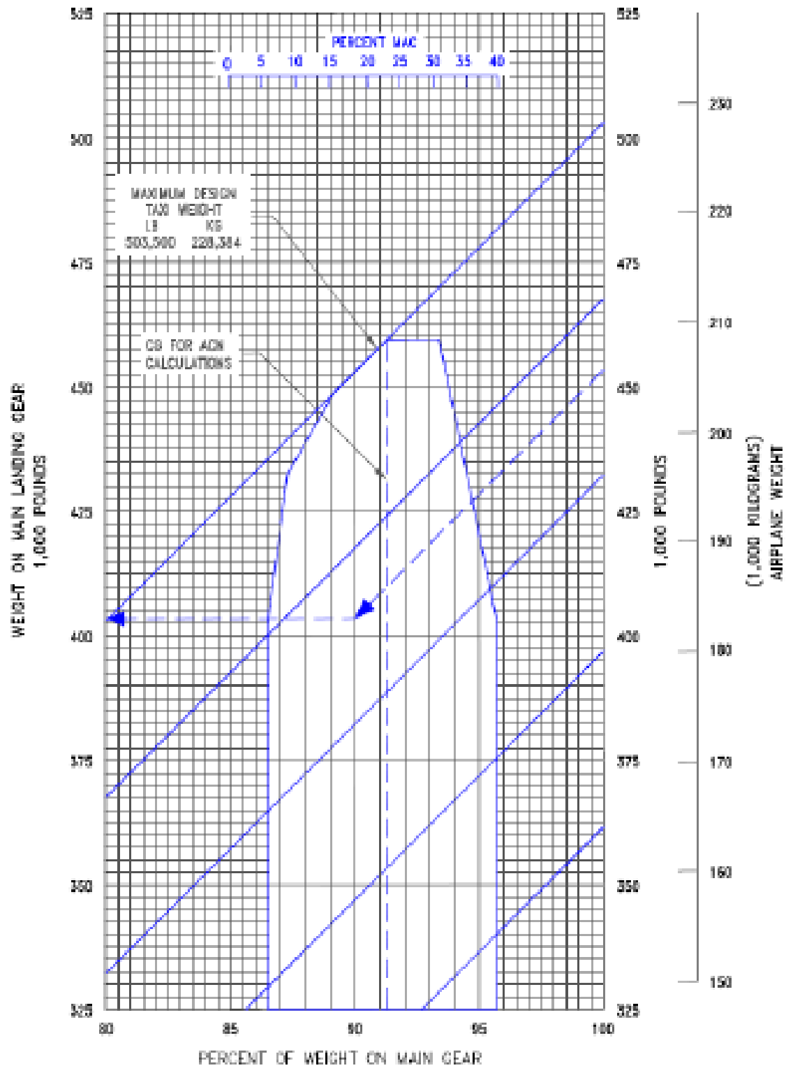
Figure 1-4. Landing gear loading on pavement - Boeing 787-8
