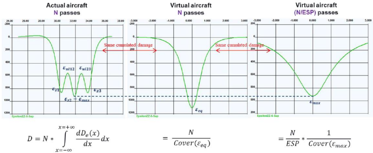
Figure A3-2. Relationship between \varepsilon_{max} , \varepsilon_{eq} and ESP
