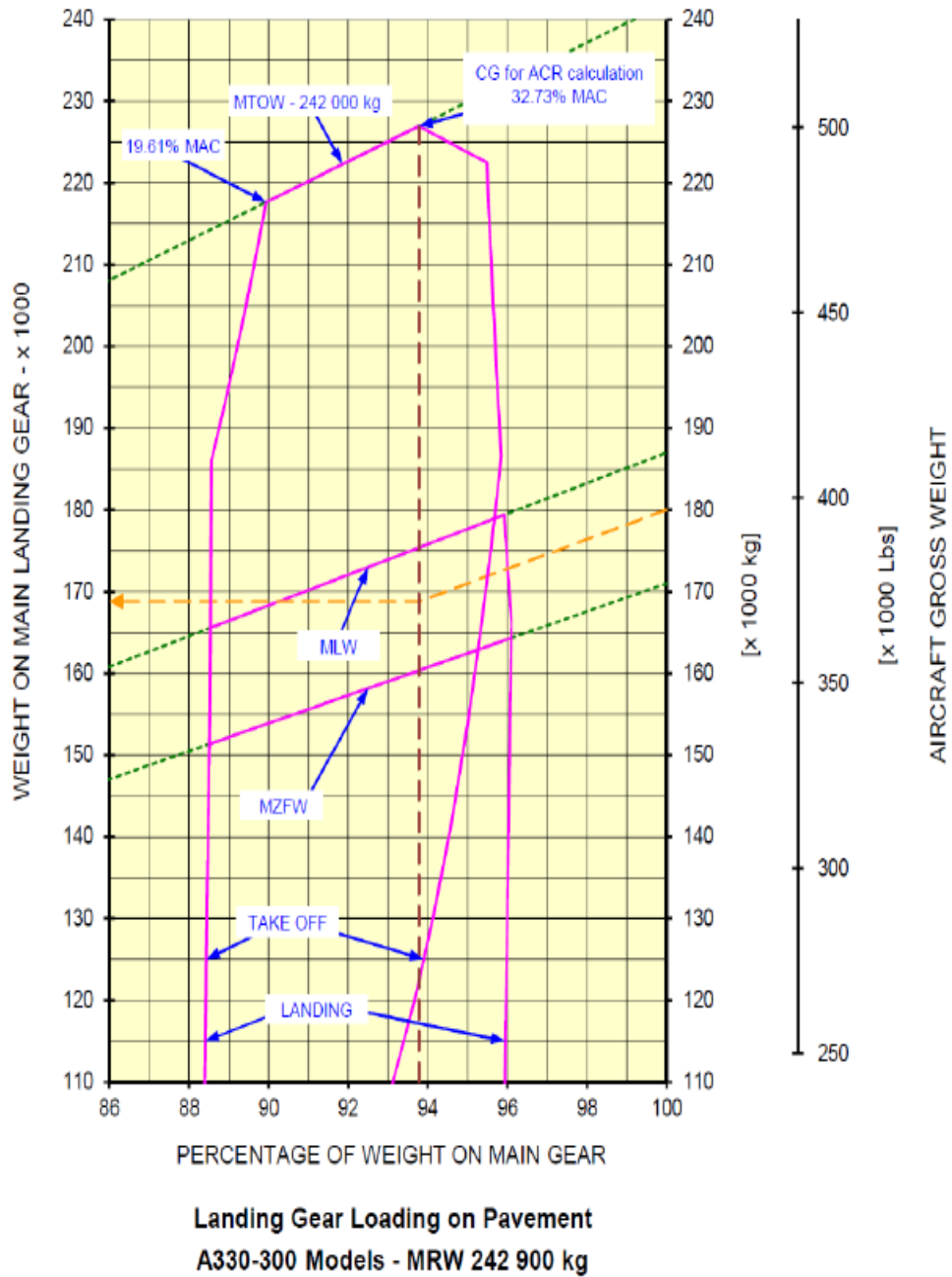
Figure 1-3. Landing gear loading on pavement - Airbus A330-300
