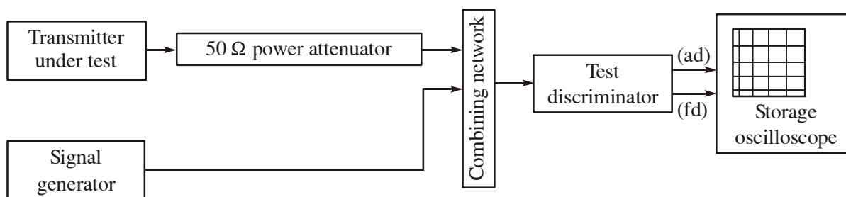
Figure 2: Measurement arrangement
